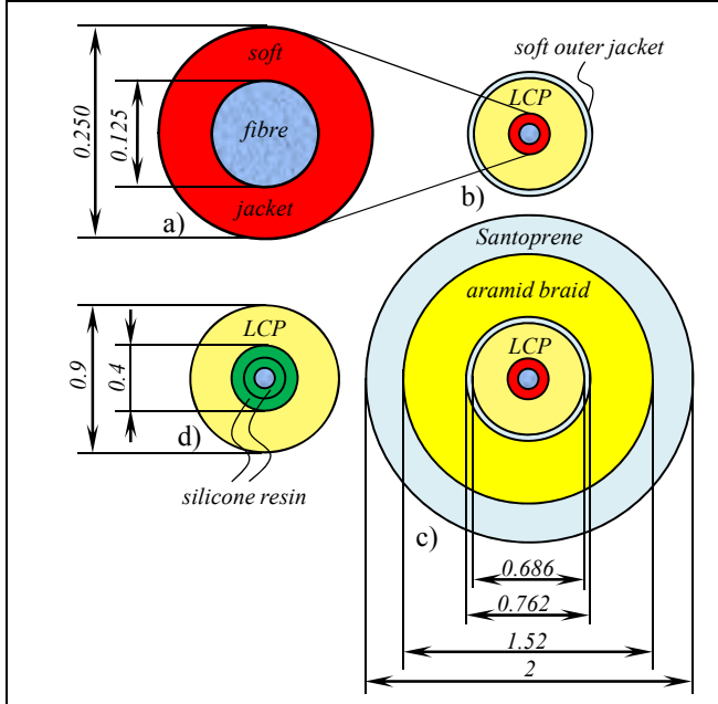
Figure 1: Tested cable types with LCP. a) 250 \mu\text{m} tight buffered, b) STFOC , c) Non-Kink STFOC , d) PSOF .
