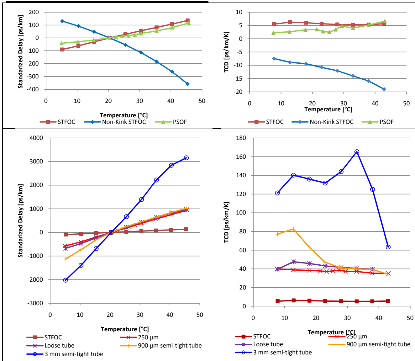
Figure 2: Measurement results of the delay drifts and the corresponding thermal coefficient of delay (TCD).
